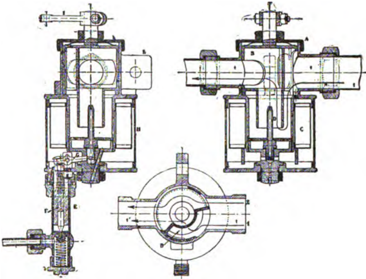
FIG. 317.—The De Dion & Bouton Vaporizer. A is the cover of the air chamber; B, the air valve; C, the float; D, the mixing chamber; E, gasoline supply; F, gasoline needle valve; G, valve controlling lever. Arrow (1) indicates course of air through mixing chamber; arrow (2), course of additional air through valve B.
